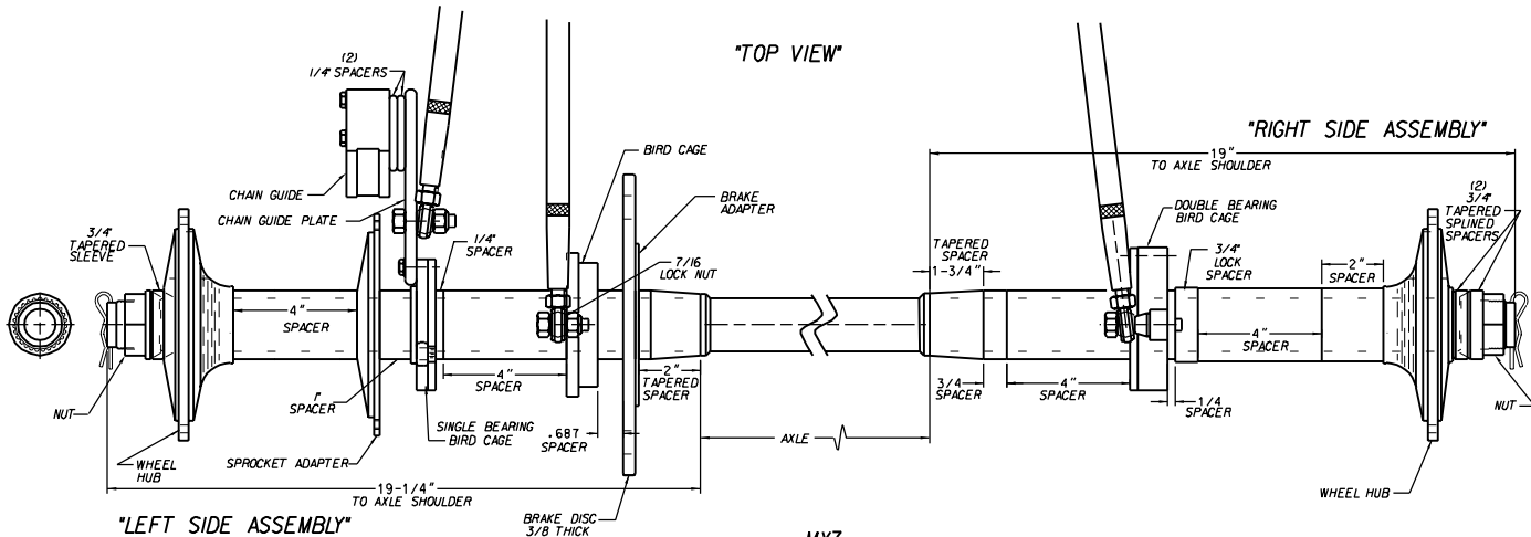
MX7 52" REAR AXLE
